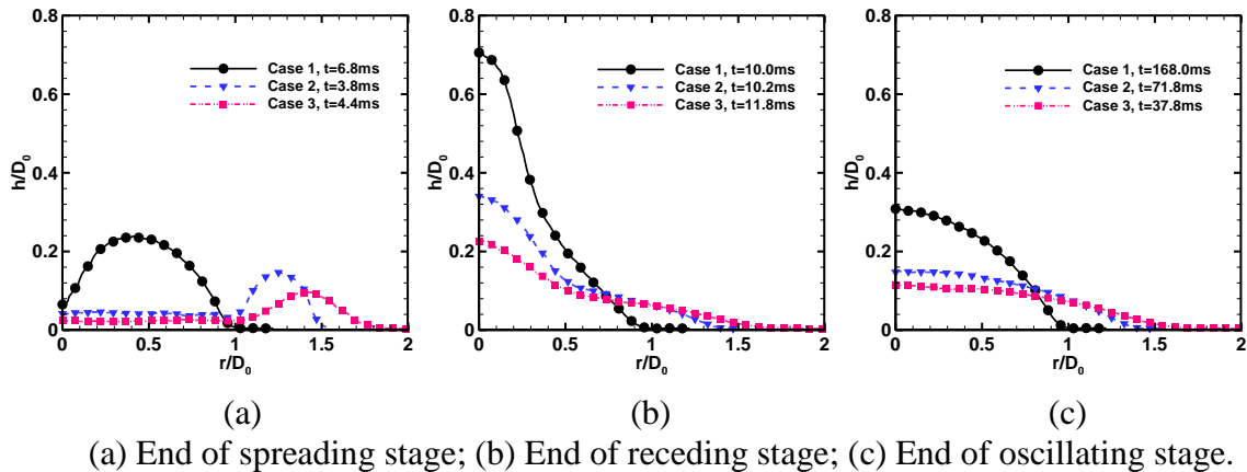
Figure 4.9 The average thickness along radius of the three distinct moments of three different impact cases
