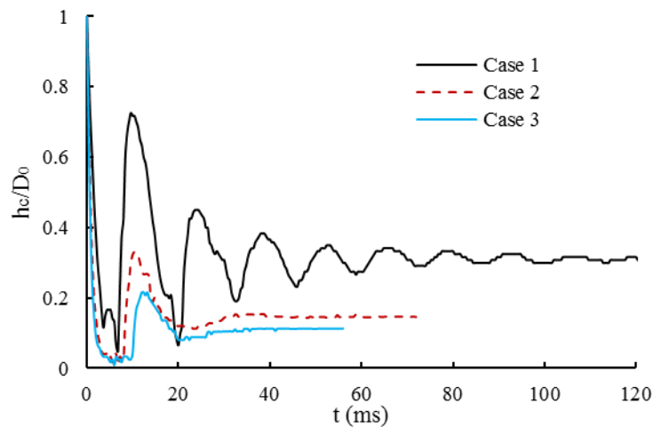
Figure 4.11 Time evolution of the droplet central point thickness under different impact conditions
