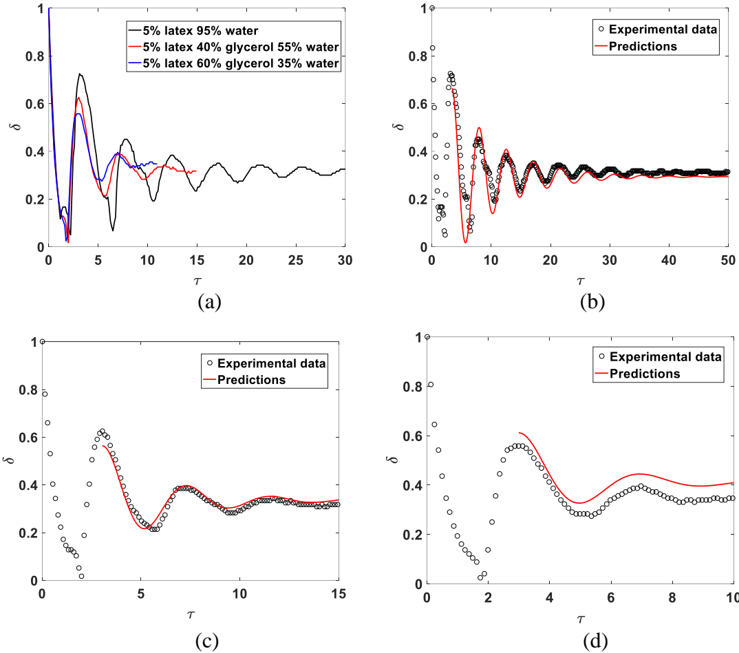
Figure 6.4 Transient variation of flattening factor \delta of droplet on the solid substrate
